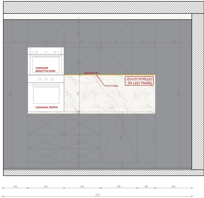
K – PRESEK KUHINJE 1
