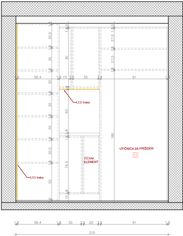
K – PRESEK KUHINJE 2
