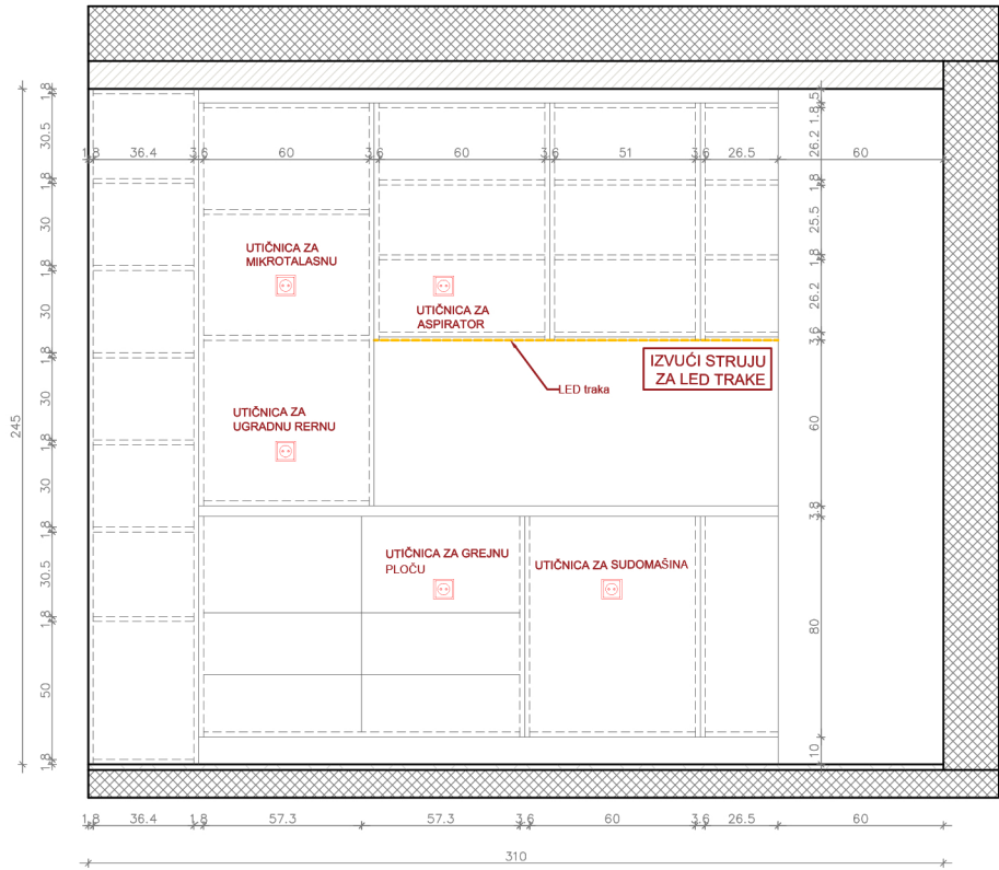
K – PRESEK KUHINJE 1
